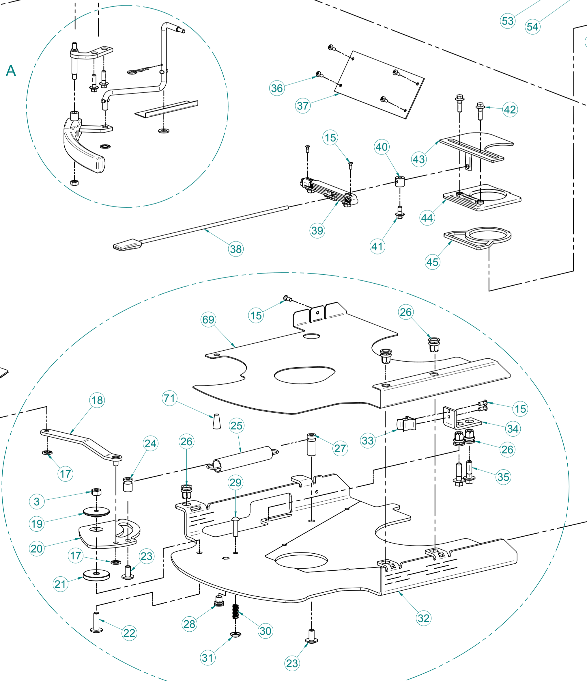
DETAIL B
